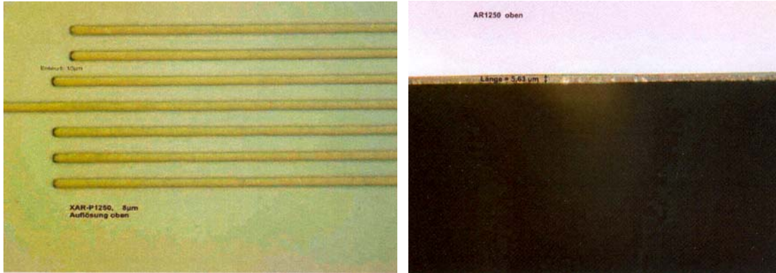
Picture 2 Dependent on the film thickness, the resolution averages 5 – 10 µm (left), the coating homogeneity is very good, and the surface is smooth (right)
