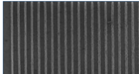
50 nm lines written on glass at a pitch of 150 nm with AR-N 7520.07 and AR-PC 5091.02
