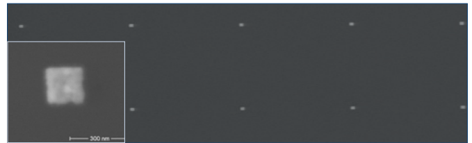
200 nm squares produced with 2-layer PMMA lift-off
